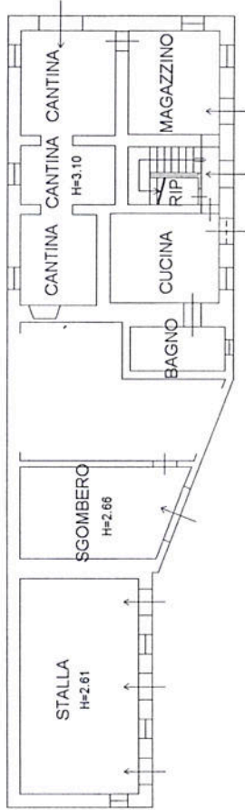
PIANO TERRA
